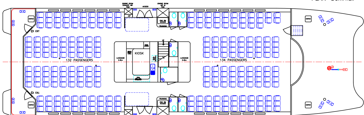
PLAN - Main Deck
