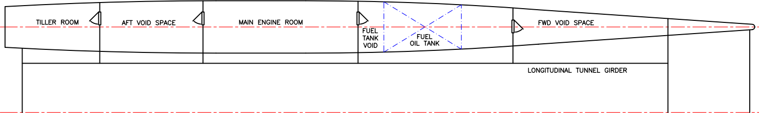
PLAN - Demi hull
