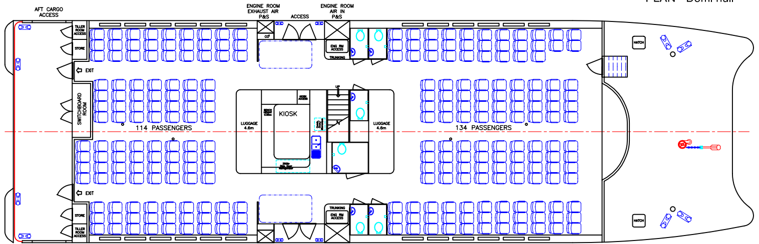
PLAN - Main Deck
