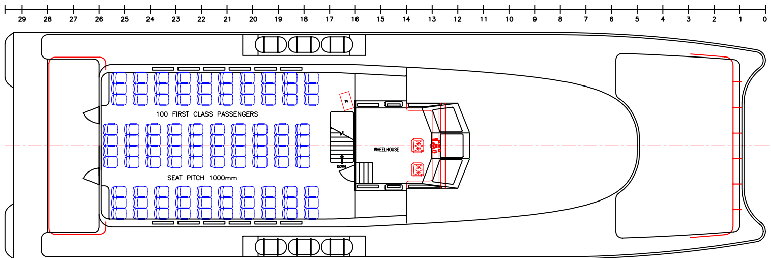
PLAN - Upper Deck
